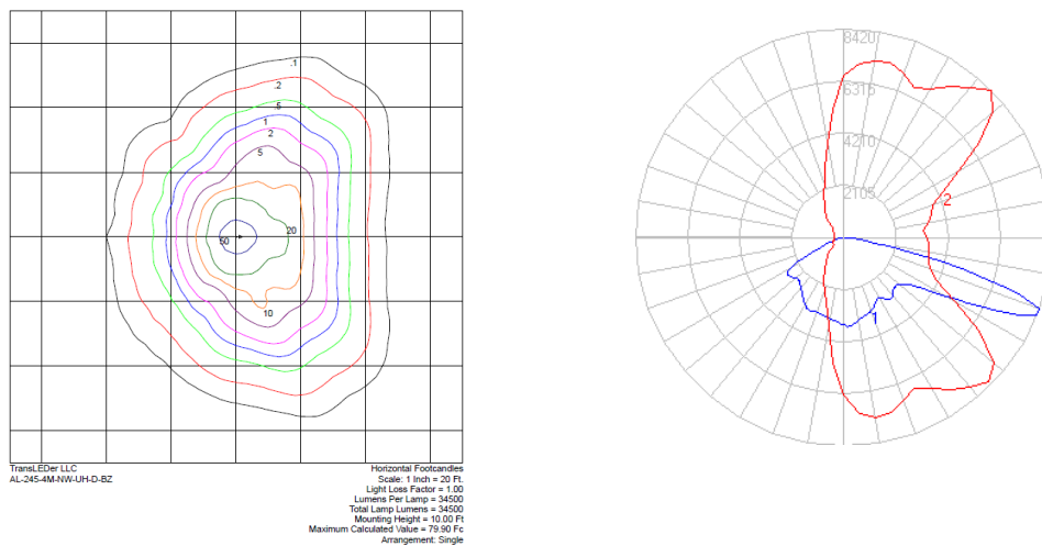
Type IV Medium Full Cutoff
