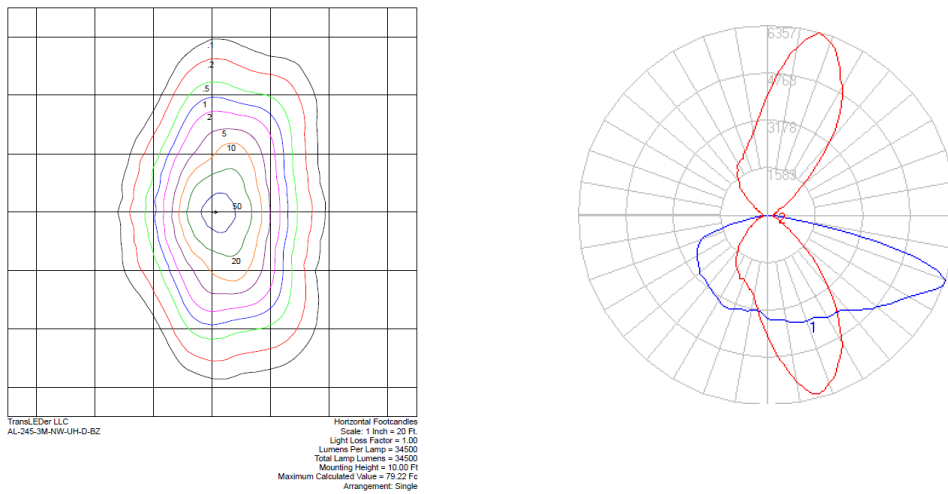
Type III Medium Full Cutoff
