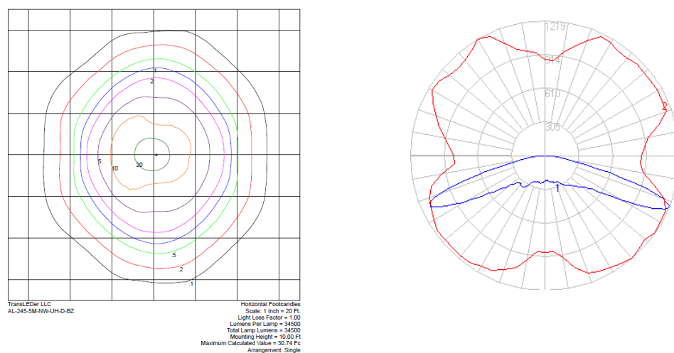
Type V Medium Full Cutoff
