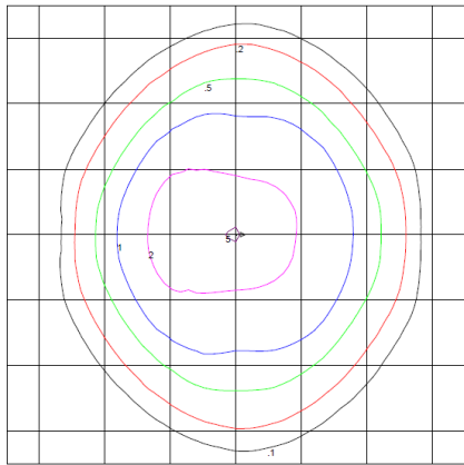
TransLEDer LLC RL-040-5M-WW-UL-D-BZ Horizontal Footcandles Scale: 1 inch = 14 Ft. Light Loss Factor = 1.00 Lumens Per Lamp = 5770 Total Lamp Lumens = 5770 Mounting Height = 10.00 Ft. Maximum Calculated Value = 5.14 Fc Arrangement: Single
