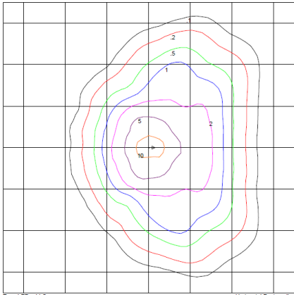
TransLEDer LLC RL-040-4M-WW-UL-D-BZ Horizontal Footcandles Scale: 1 inch = 13 Ft. Light Loss Factor = 1.00 Lumens Per Lamp = 5770 Total Lamp Lumens = 5770 Mounting Height = 10.00 Ft. Maximum Calculated Value = 13.36 Fc Arrangement: Single
