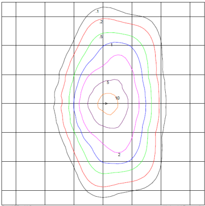
TransLEDer LLC RL-040-3M-WW-UL-D-BZ Horizontal Footcandles Scale: 1 inch = 13 Ft. Light Loss Factor = 1.00 Lumens Per Lamp = 5770 Total Lamp Lumens = 5770 Mounting Height = 10.00 Ft. Maximum Calculated Value = 13.25 Fc Arrangement: Single
